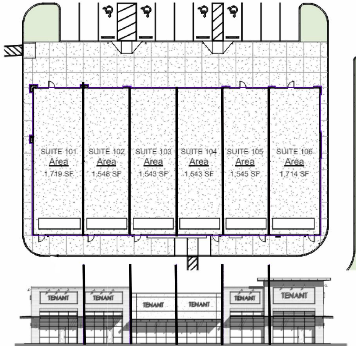
BUILDING 4 - FLOOR PLAN/DIMENSIONS
